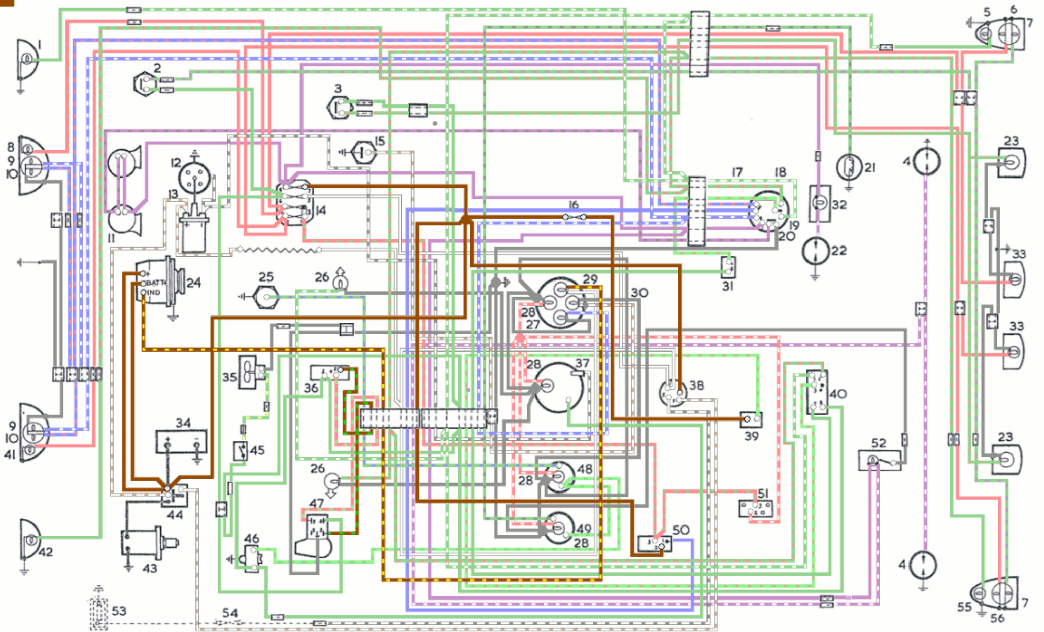
Fig. 10.31 Wiring diagram (UK) – 1978 models
