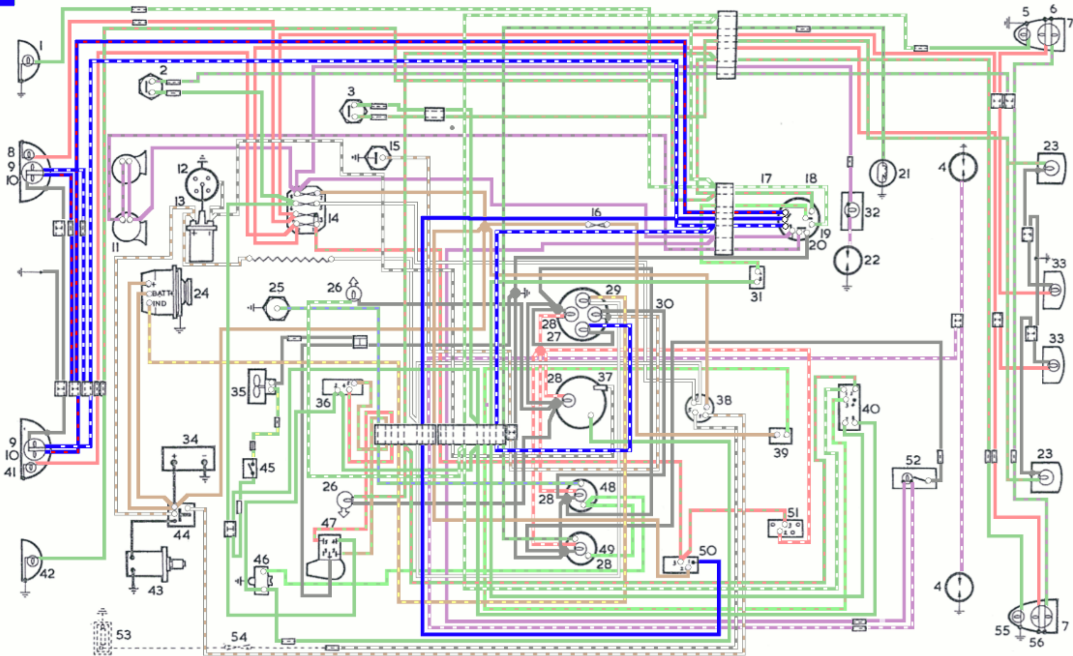
Fig. 10.31 Wiring diagram (UK) – 1978 models
